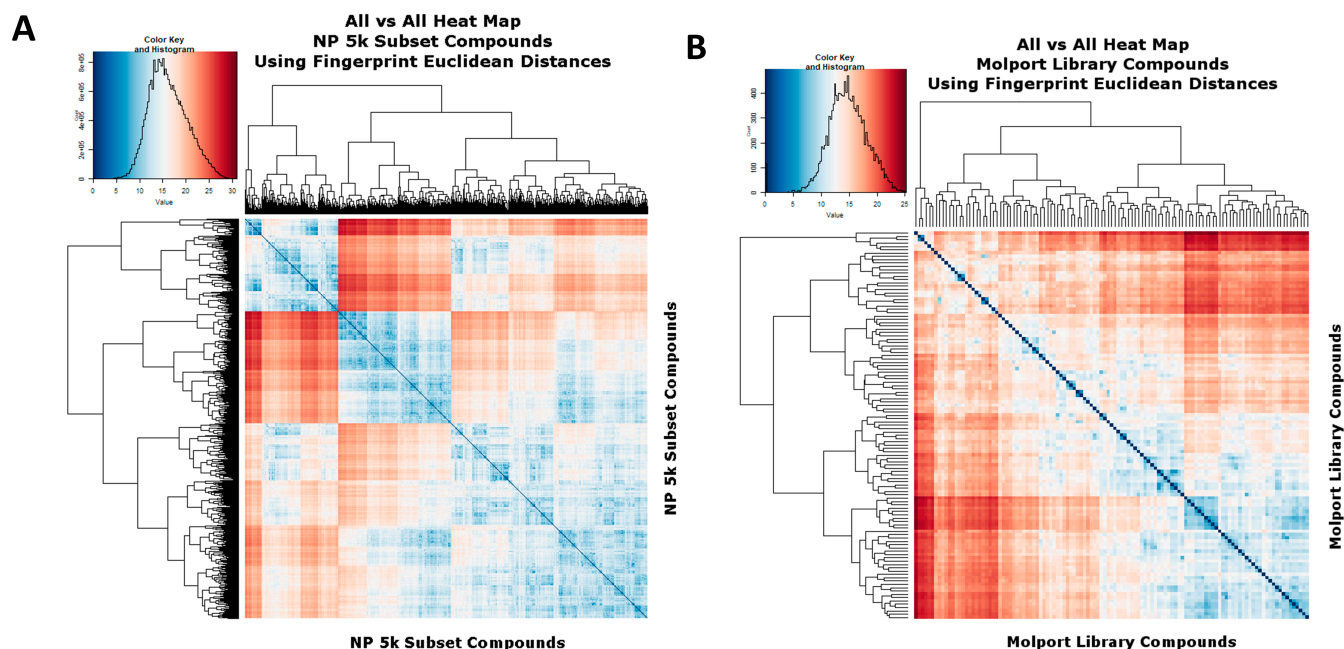
Figure 4. Heat map analyses of (A) The 5000-molecule subset, based on their Euclidean distances, as described in the text. Analyses and displays were otherwise as per Figures 2 and 3. (B) The 117-molecule subset, based on their Euclidean distances, as described in the text. Analyses and displays were otherwise as per Figures 2 and 3.
