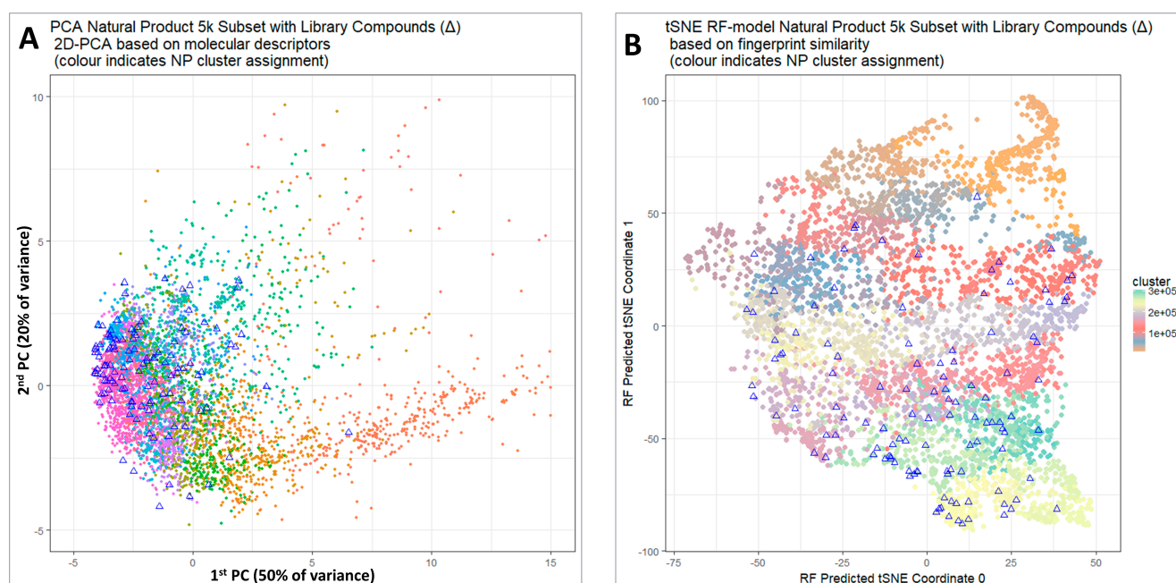
Figure 2. (A) Visualisation of the coverage of natural product(-like) space when molecules are selected from individual clusters. Principal components analysis was performed after normalizing to unit variance using a standard KNIME workflow. 5000 molecules are shown for purposes of visualization, and the 118 molecules closest to cluster centres that fulfilled our other criteria are indicated with triangles. (B) A t-SNE plot of the same data as in Figure 2A.
