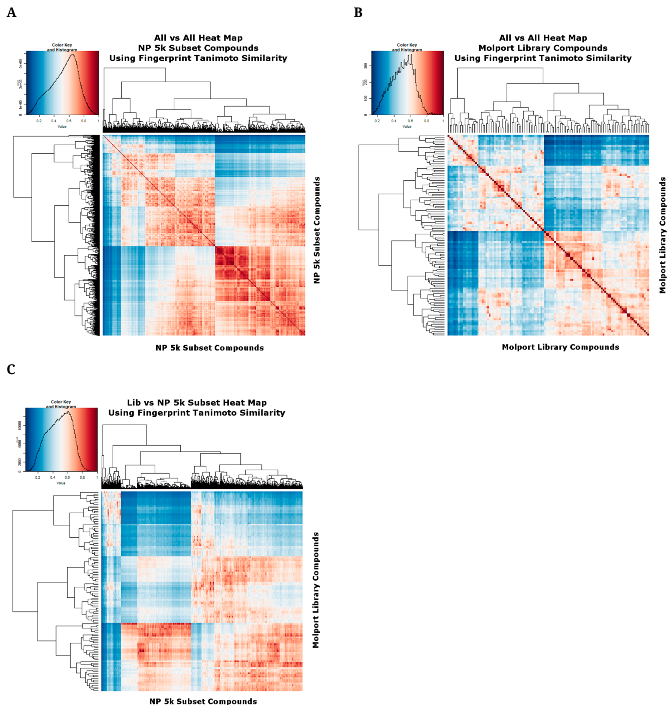
Figure 3. Heat map analyses of (A) The 5000-molecule subset and (B) The 117-molecule subset, based on their Tanimoto similarities. The analyses used the same workflows as those described in [32]. (C) The 5000-molecule subset versus the 117-molecule subset, based on their Tanimoto similarities. The analyses used the same workflows as those described in [32].
